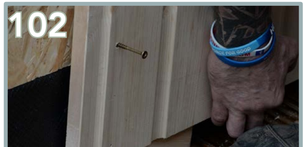
Use 6 x 80mm screws to secure each cladded panel (3 screws down each side). Screw through the batten on the panel and into the wall behind. Leave the screws slightly out in case of adjustment.
