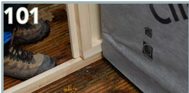
Repeat the same process for the second Back Panel (AX). Use a rubber mallet to softly knock the second back panel into the first, so the T&G Panels interlock.
