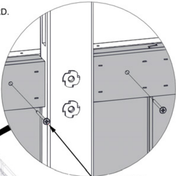
382 (x36) SCREW - 1 3/4"
