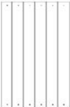
WP01 WALL PANEL - W2A03998 (x3) 1 1/16"x19 15/16"x30 9/16" (27x507x777)
