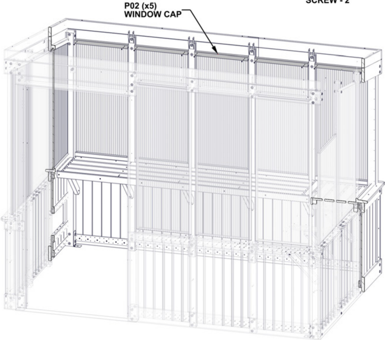
391 (x10) SCREW - 2"
