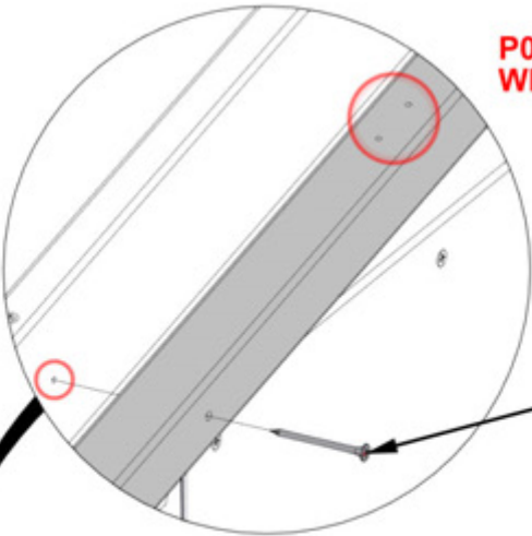
391 (x8) SCREW - 2"
