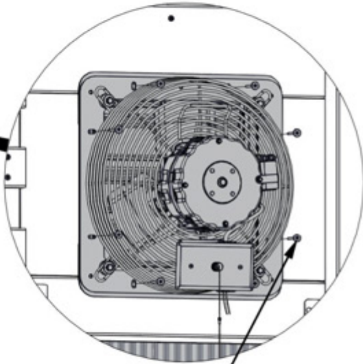
1203 (x8) SCREW - 1 1/4"
