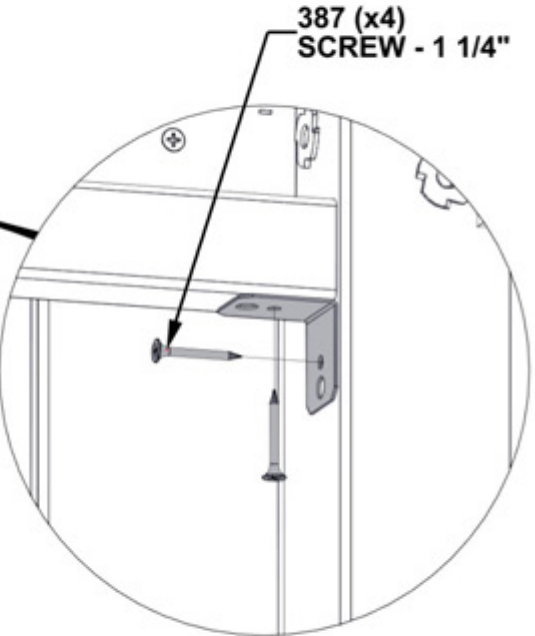
555 (x2) L BRACKET BLK
