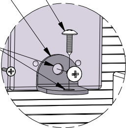
061 (x2) L BRACKET GREEN 32x51 083 (x4) SCREW - 14x3/4"
