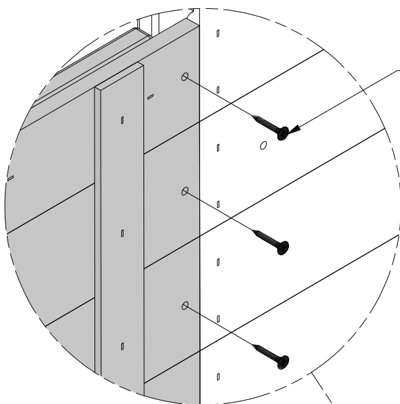
385 (x12) SCREW - 1"
