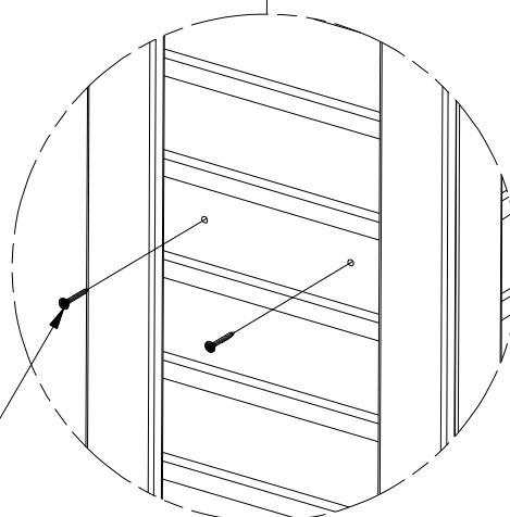
387 (x4) SCREW - 1 1/4"
