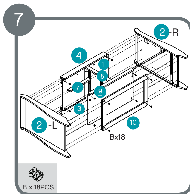
Assemble locking nuts B x 18.
